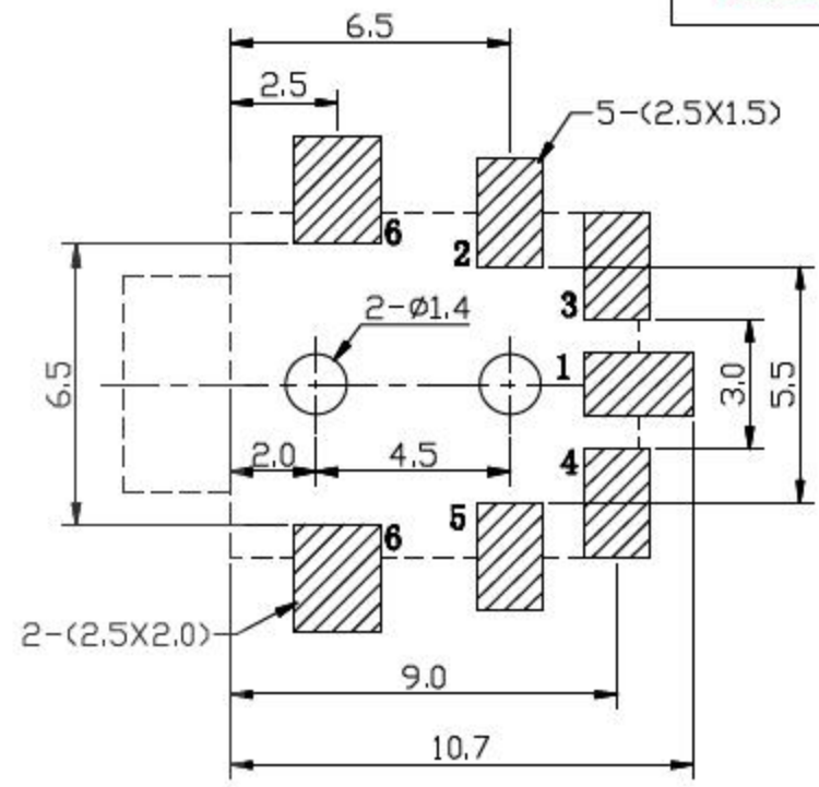
PCB LAYOUT MOUNTING PATTERN TOP VIEW
