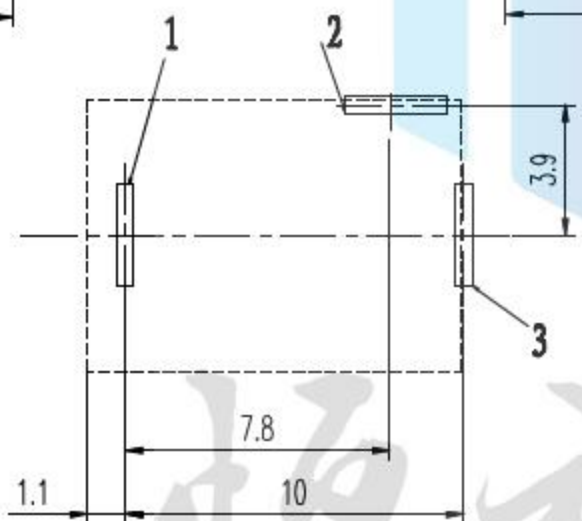
P.C.B HOLE LAYOUT BOTTOM VIEW
