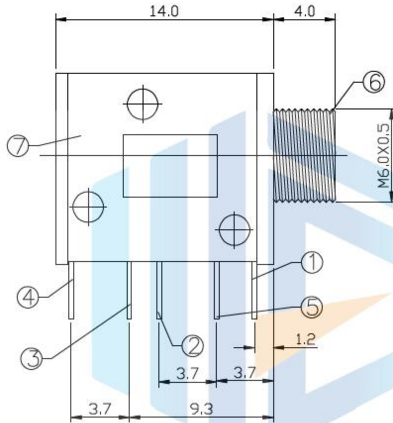
SCHMATIC
