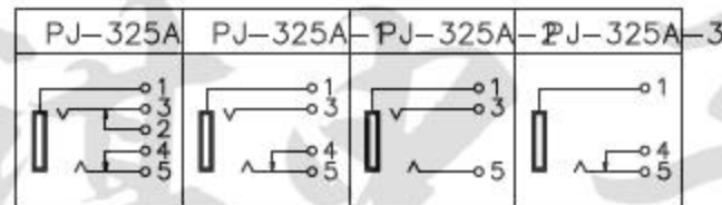
SCHMATIC
