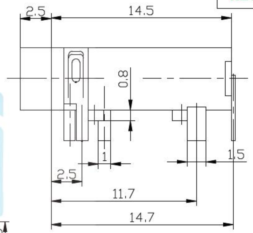
P.C.B LAYOUT TOP VIEW
