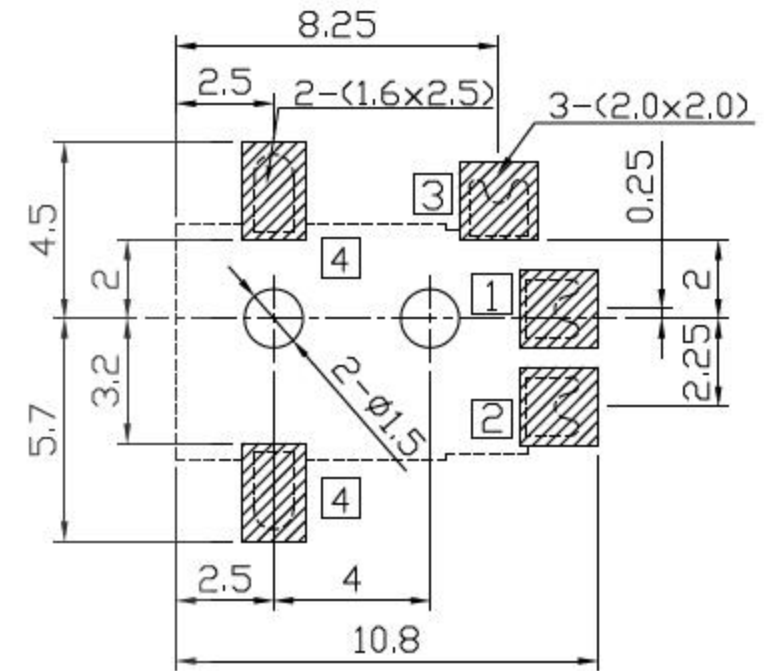
RECOMMENDED P.C.B. LAYOUT UNSPECIFIED TOLERANCE: ±0.05
