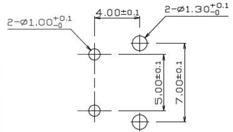
P.C.B MOUNTING HOLE DIMENSION
