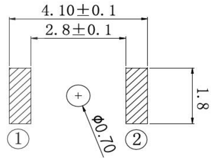
PCB. 焊接图 PCB. WELDING DRAWING
