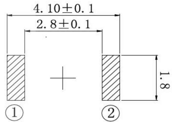
PCB. 焊接图 PCB. WELDING DRAWING
