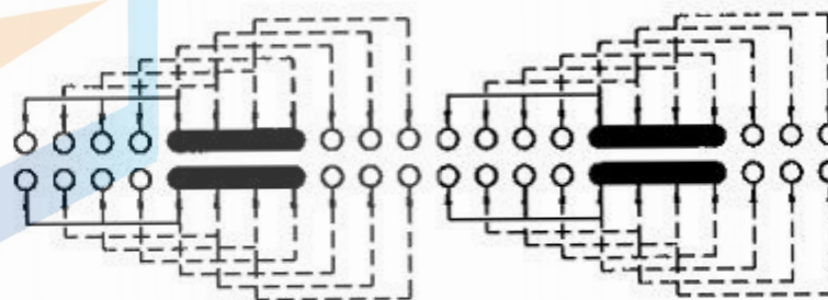
SCHEMATIC (SHORTING)
