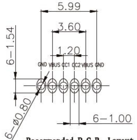
Recommended P.C.B. Layout Unspecified tolerance: \pm 0.05 (Top view)
